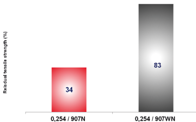
Comparison of residual strength after dry heat treatment of the FireRetard® types 9xxN and 9xxWN
